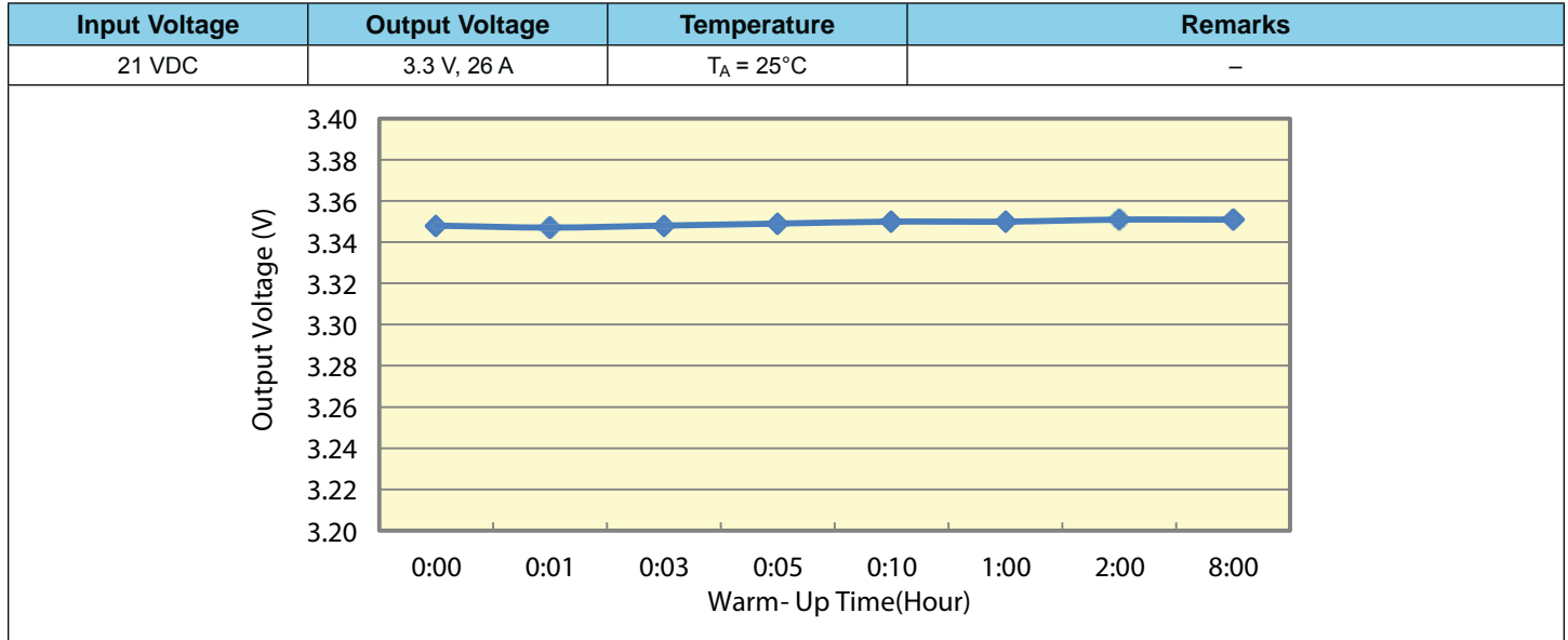
Figure 3. Warm-Up Drift
