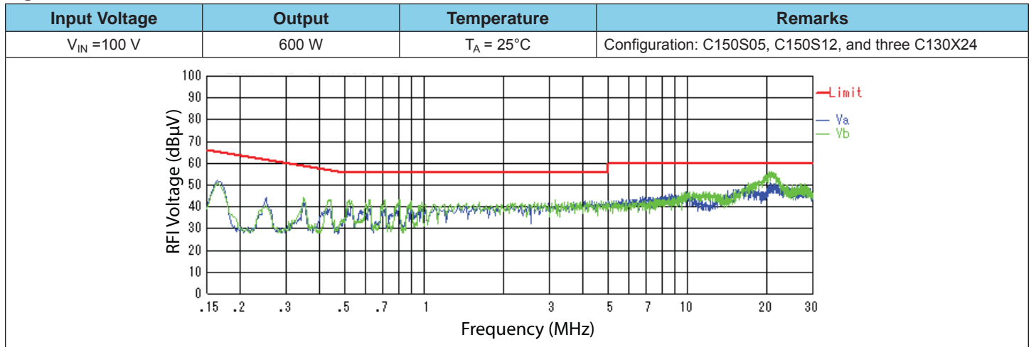
Figure 9. Conduction Noise 100 V/600 W
