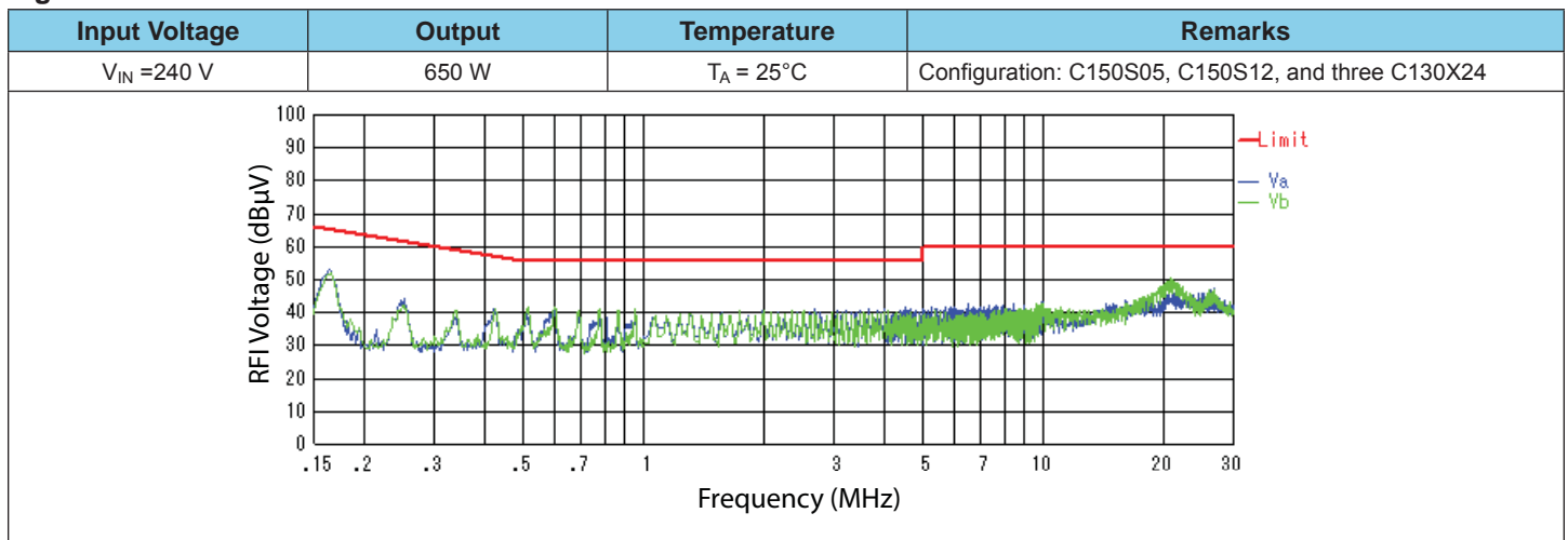
Figure 10. Conduction Noise 240 V/650 W
