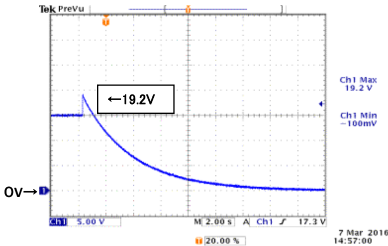
図18 過電圧波形 Fig.18 Over Voltage Waveform
