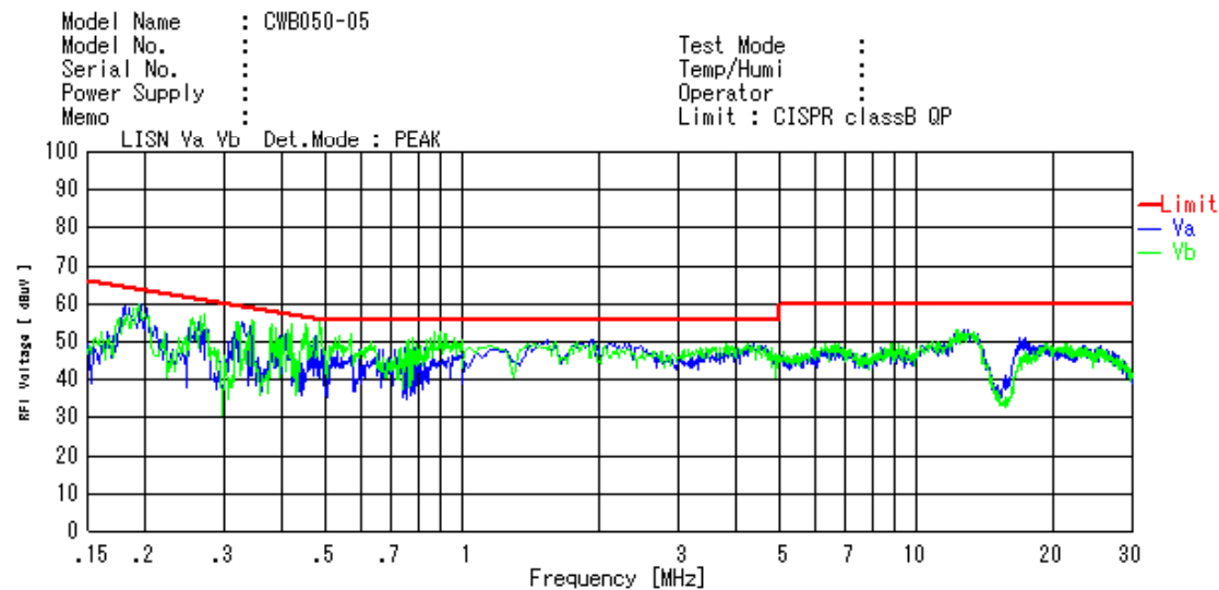
図20 雑音端子電圧 Fig.20 Conduction Noise Waveform
