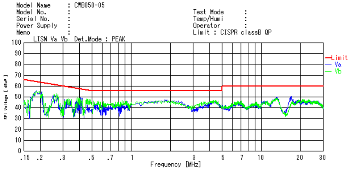
図19 雑音端子電圧波形 Fig.19 Conduction Noise Waveform
