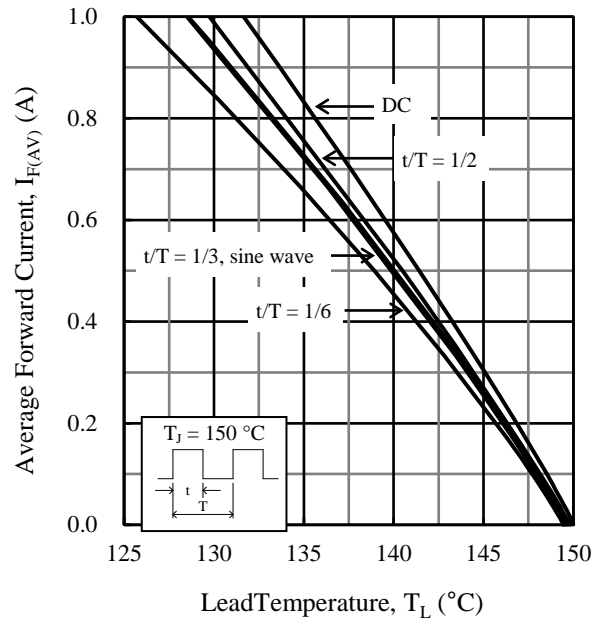
Figure 3. T_L vs. I_{F(AV)} Typical Characteristics ( V_R = 600 V)
