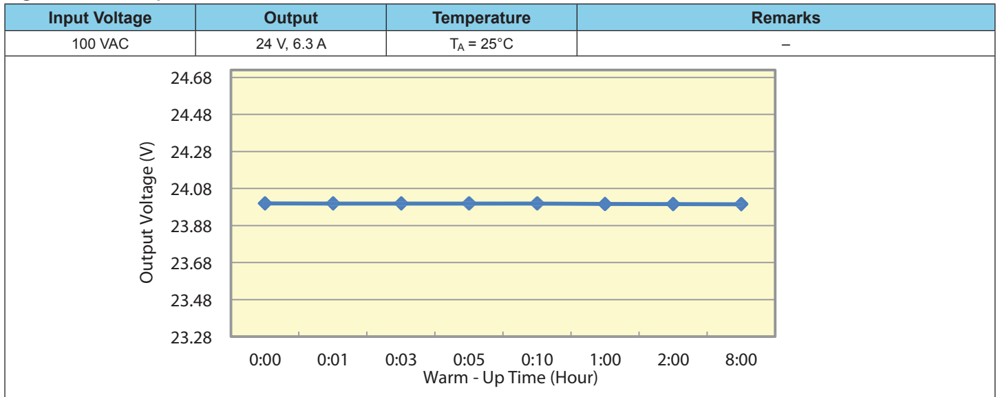
Figure 9. Warm-Up Drift
