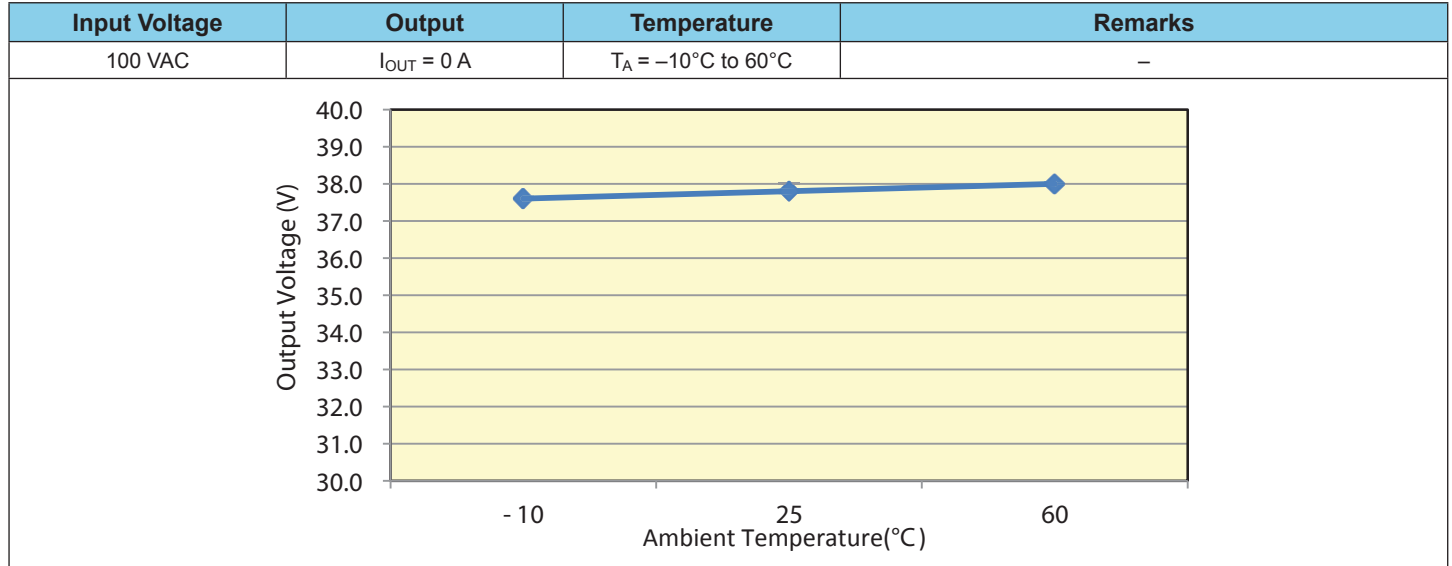
Figure 15. Overvoltage Protection (By Temperature)
