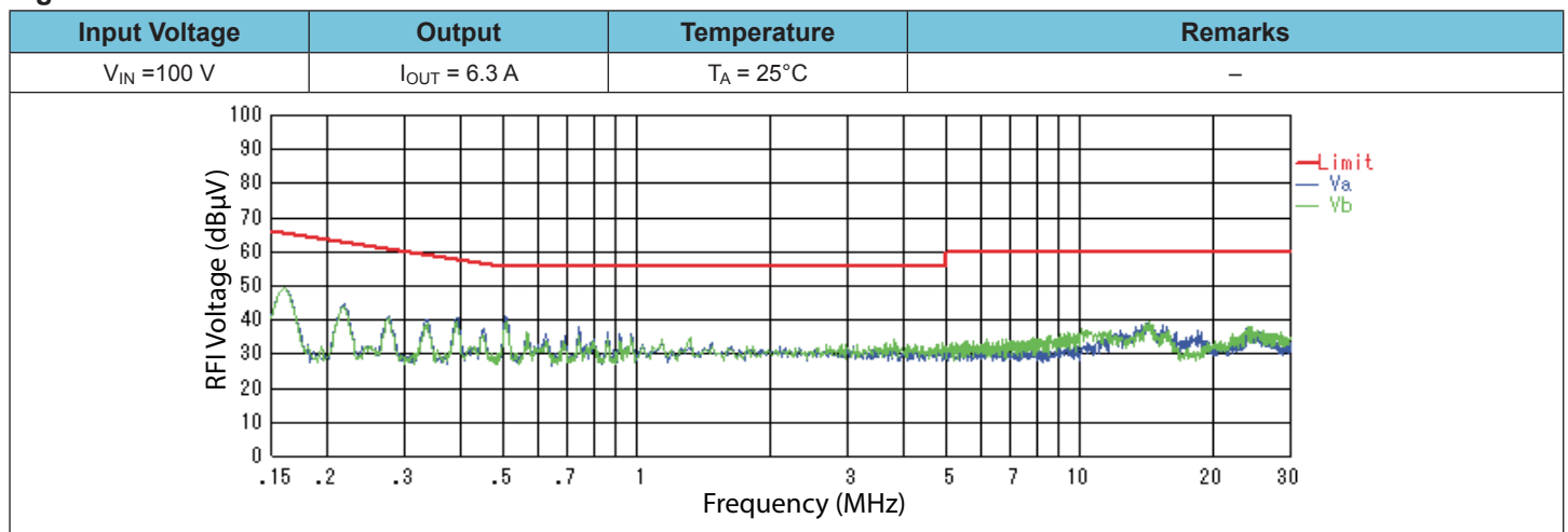
Figure 18. Conduction Noise 100 V
