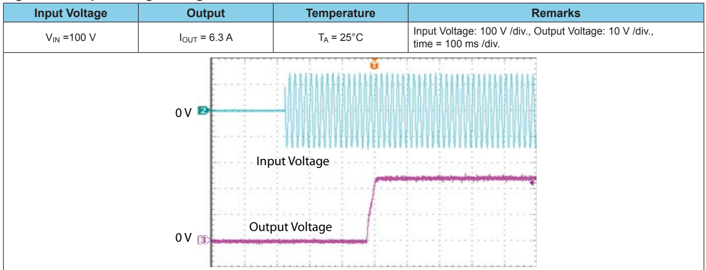
Figure 12. Output Voltage Rising
