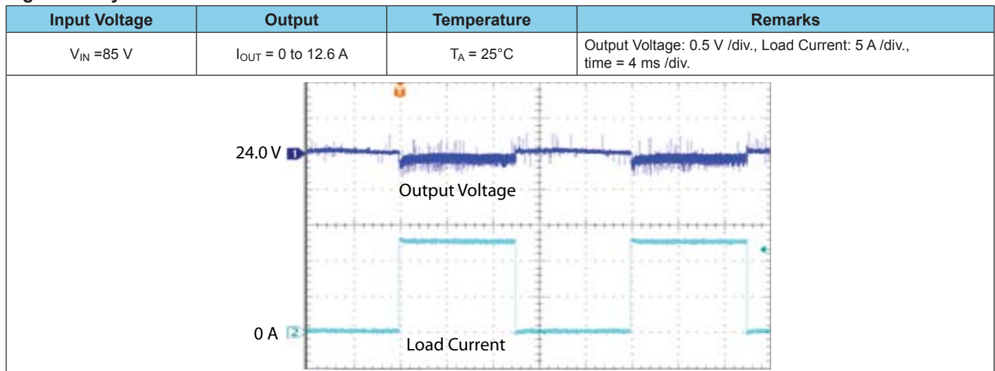
Figure 20. Dynamic Load
