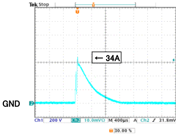
図16 突入電流波形 Fig.16 Inrush Current Waveform
