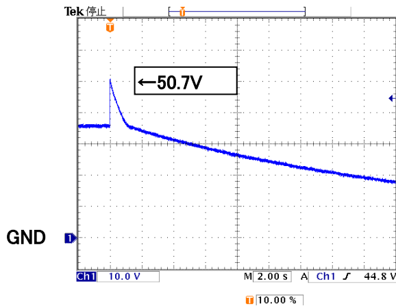
図17 過電圧波形 Fig.17 Over Voltage Waveform
