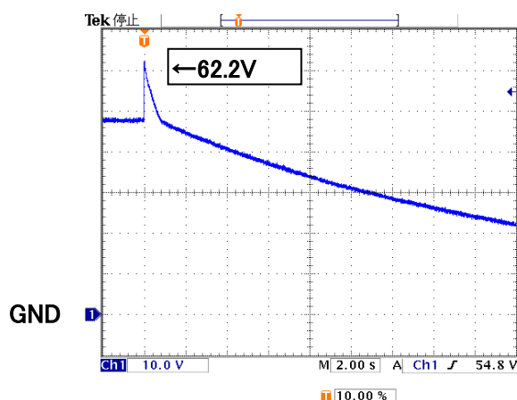
図17 過電圧波形 Fig.17 Over Voltage Waveform
