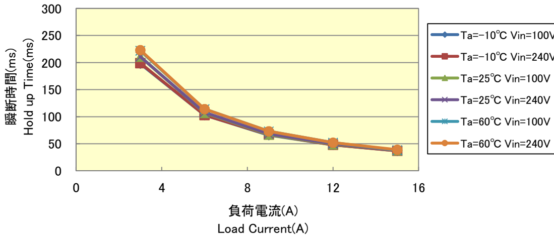
Fig.12 Hold up time Characteristics (vs Load Current)
