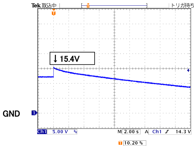
図17 過電圧波形 Fig.17 Over Voltage Waveform
