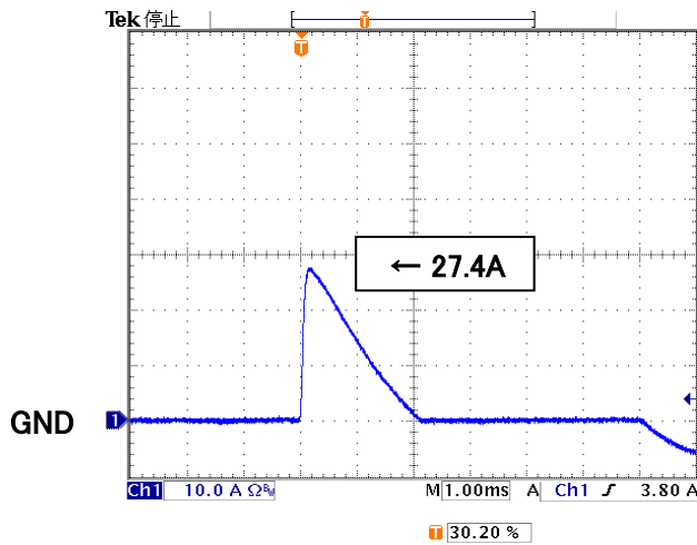
図16 突入電流波形 Fig.16 Inrush Current Waveform
