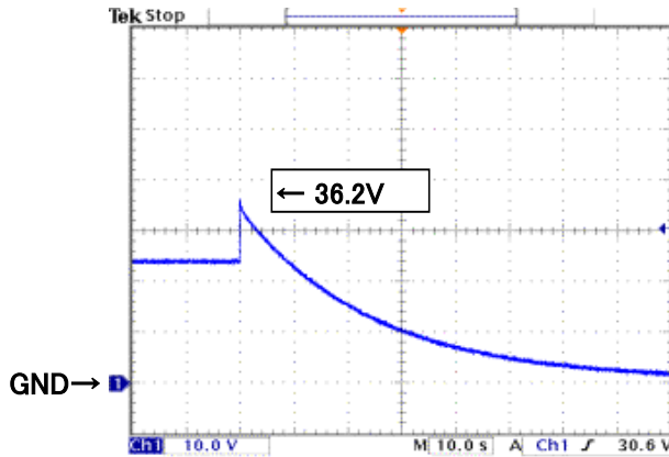
図17 過電圧波形 Fig.17 Over Voltage Waveform
