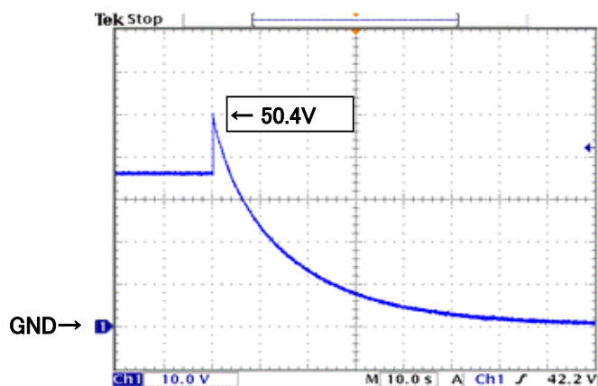
Fig.17 Over Voltage Waveform
