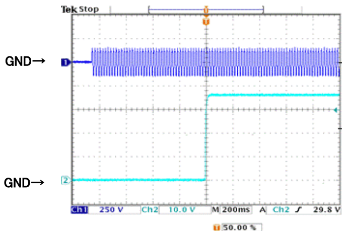
Fig.14 Output Voltage Rising Waveform
