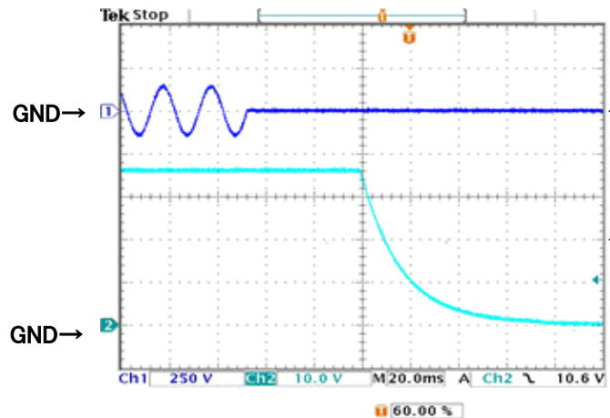
Fig.15 Output Voltage Falling Waveform
