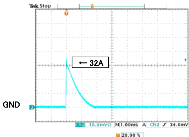
図16 突入電流波形 Fig.16 Inrush Current Waveform
