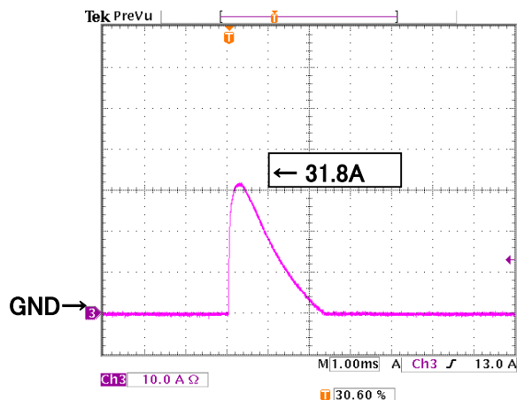
図16 突入電流波形 Fig.16 Inrush Current Waveform
