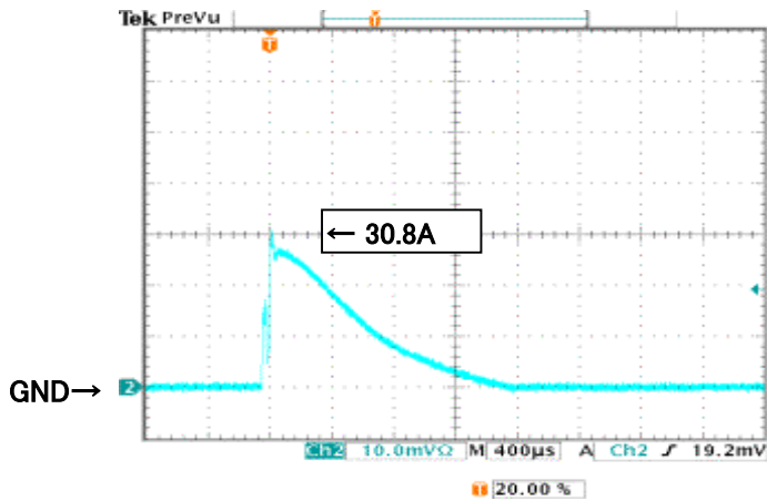
図16 突入電流波形 Fig.16 Inrush Current Waveform
