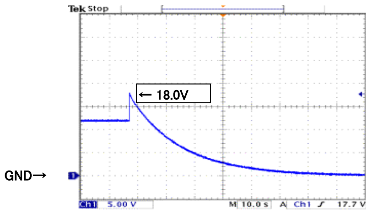
図17 過電圧波形 Fig.17 Over Voltage Waveform
