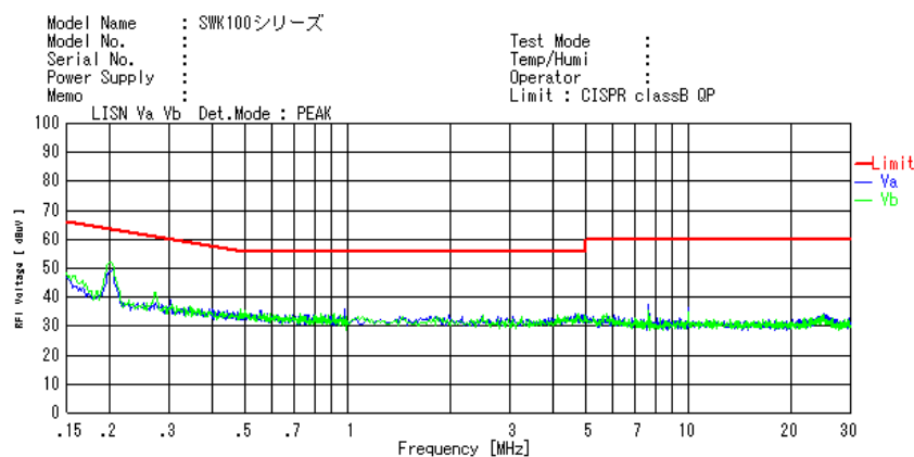
Fig.18 Conduction Noise Waveform Reference data
