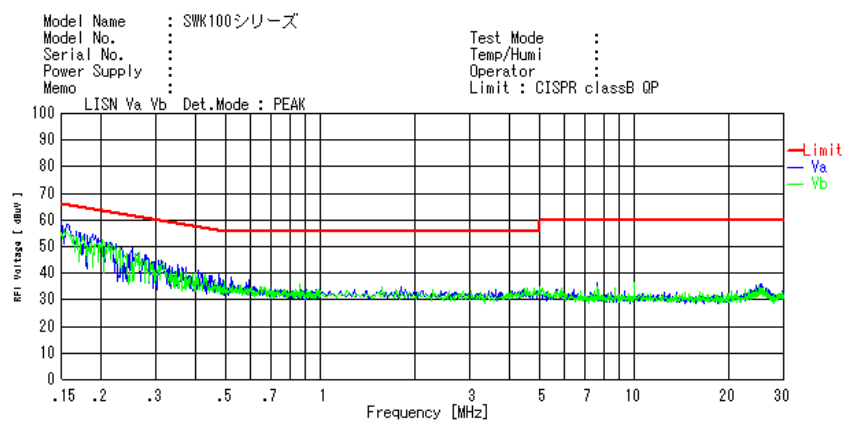
Fig.19 Conduction Noise Waveform Reference data
