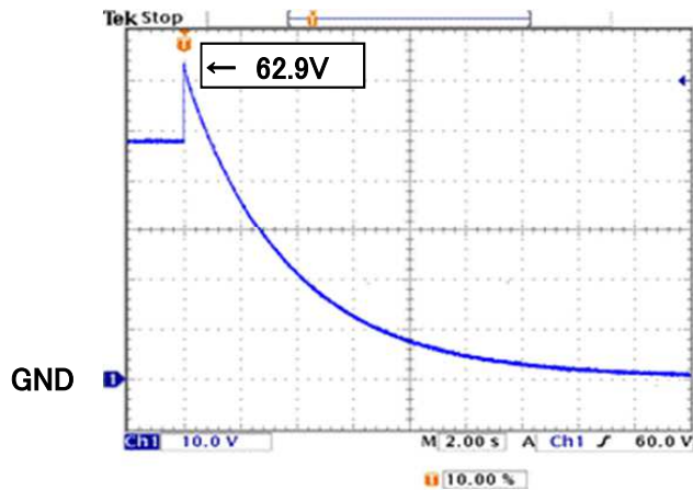
図17 過電圧波形 Fig.17 Over Voltage Waveform
