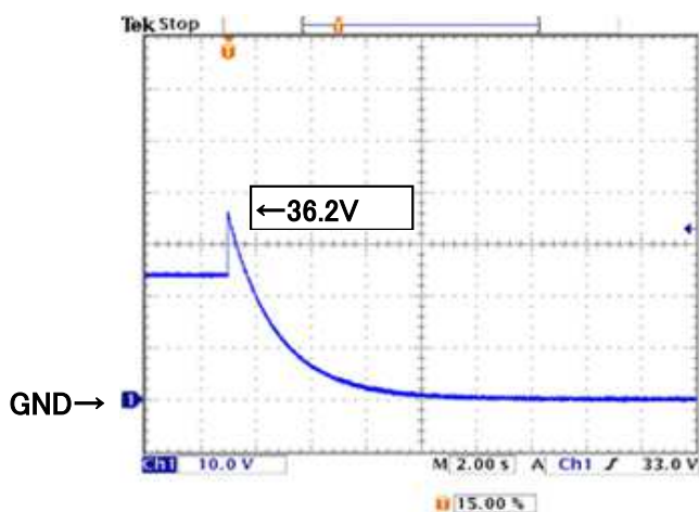
図17 過電圧波形 Fig.17 Over Voltage Waveform
