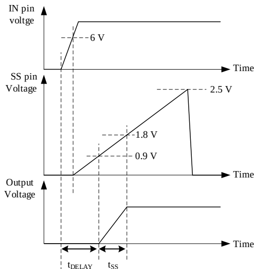
Figure 11-3. Soft Start Operation Waveform
