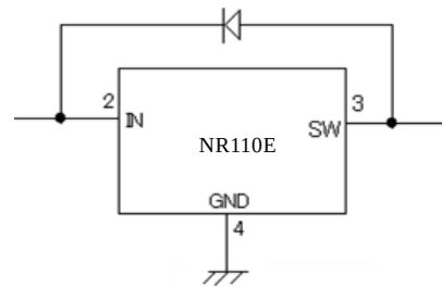
Figure 12-12. When the SW pin voltage becomes higher than the IN pin voltage
