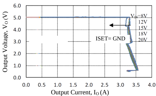
Figure 5-12. Overcurrent Protection
