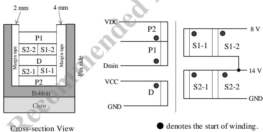
Figure 32. Winding Structure
