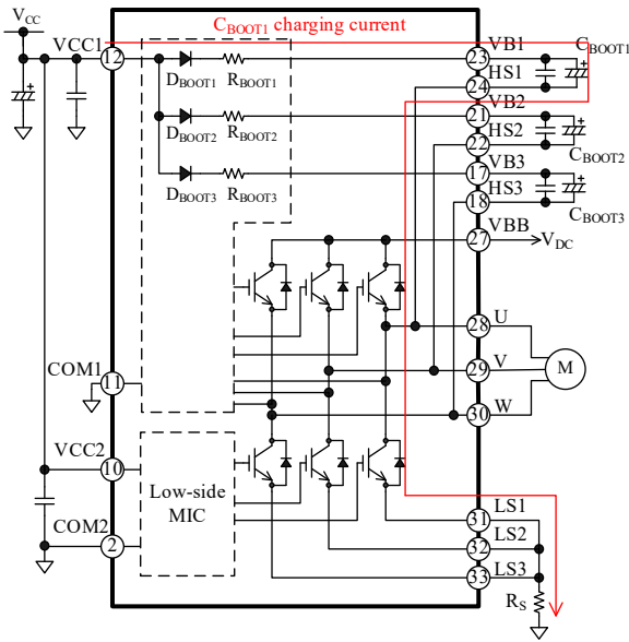
Figure 12-1. Bootstrap Circuit
