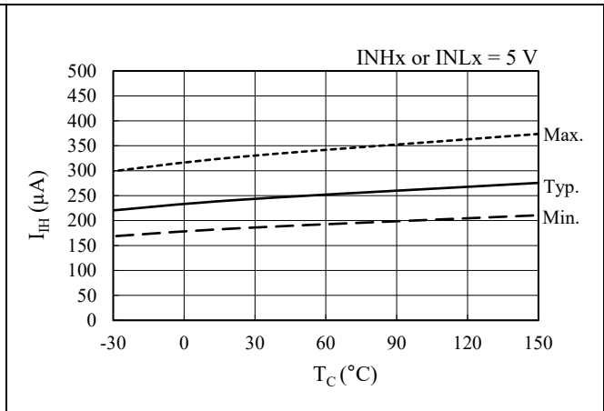
Figure 15-13. Input Current at High Level (HINx or LINx), I_H vs. T_C
