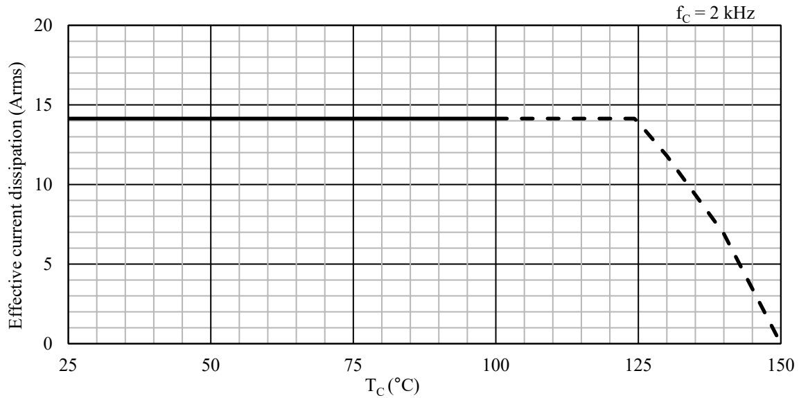
Figure 15-40. Allowable Effective Current ( f_c = 2\text{ kHz} ): SCM2007MKF
