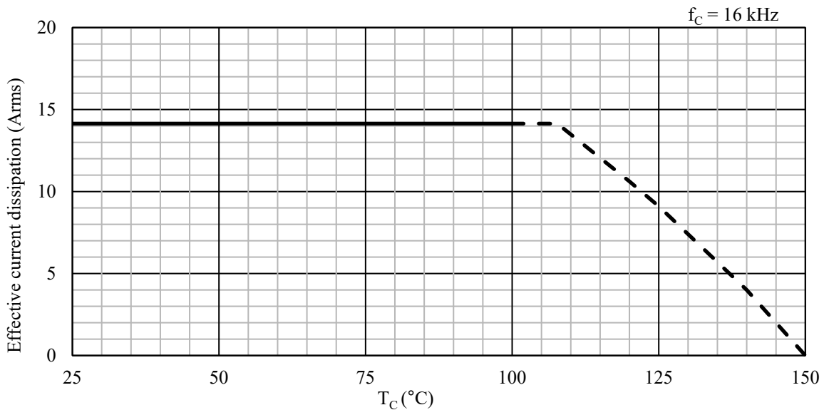
Figure 15-41. Allowable Effective Current ( f_c = 16\text{ kHz} ): SCM2007MKF
