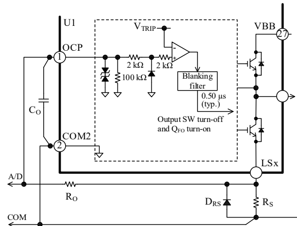
Figure 12-19. Internal Circuit Diagram of OCP Pin and Its Peripheral Circuit
