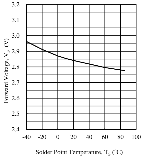
Figure 5. V_F vs. T_S ( I_F = 65 mA)
