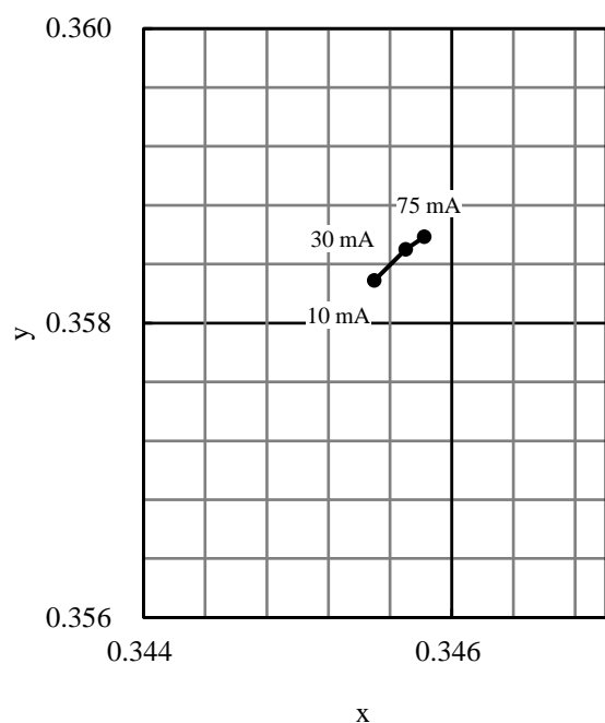
Figure 8. I_F vs. Chromaticity ( T_A = 25\text{ }^{\circ}\text{C} )
