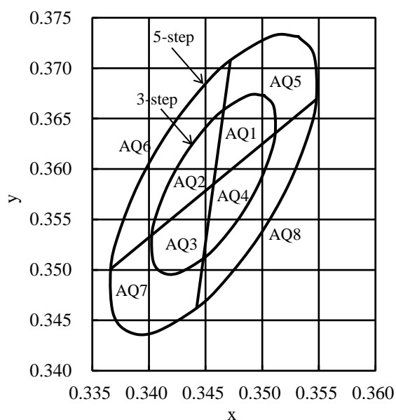
Figure 2. Chromaticity Diagram
