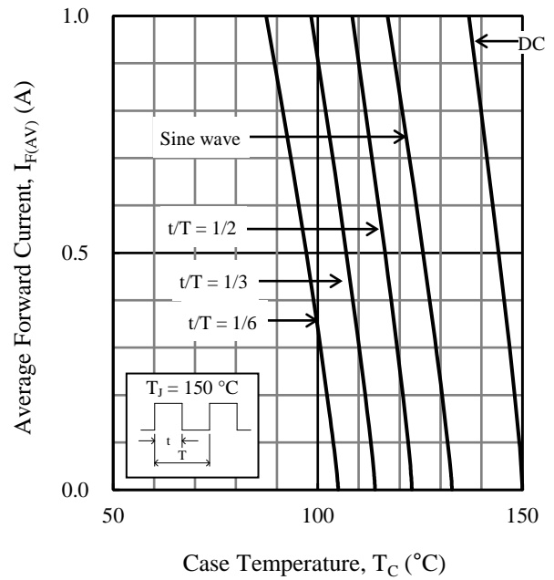
Figure 2. T_C vs. I_{F(AV)} Typical Characteristics ( V_R = 90\text{ V} )
