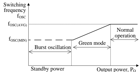
Figure 9-8. Relationship between P_O and f_{OSC}
