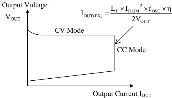
Figure 10-9 CV/CC characteristics
