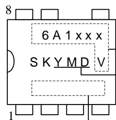
STR6A100xV
