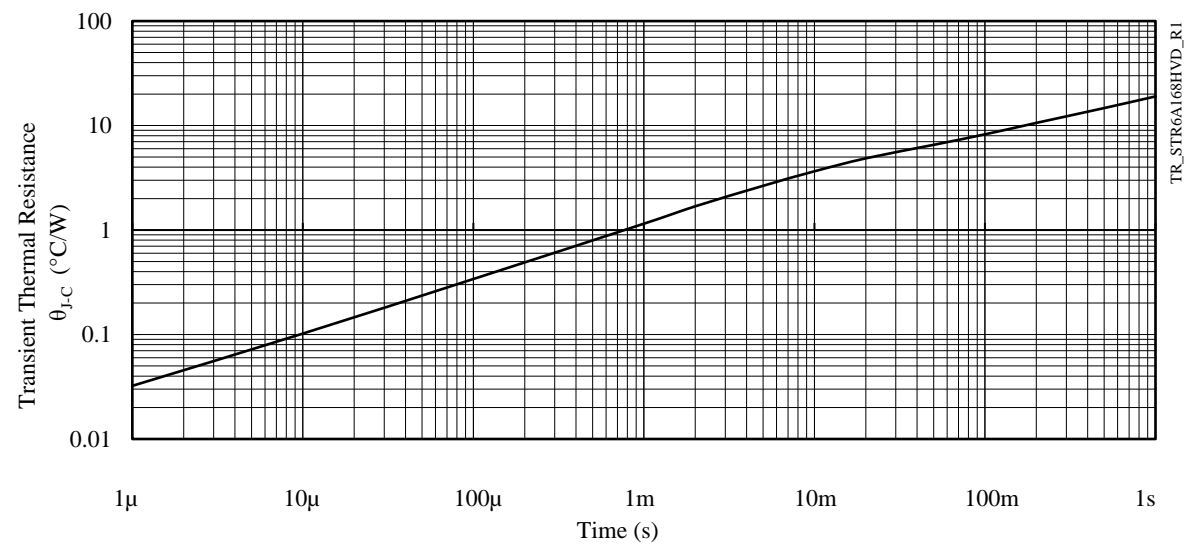
Figure 3-12. STR6A168HV/HVD Transient Thermal Resistance Curve
