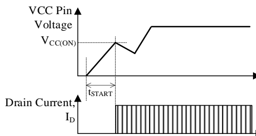
Figure 9-2. Startup Operation
