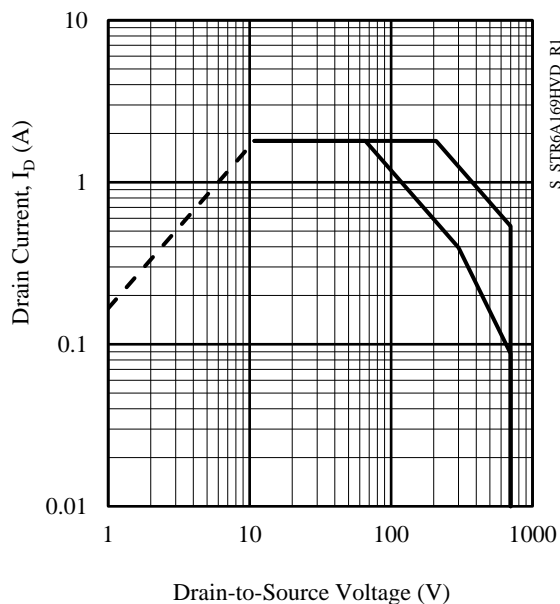
Figure 3-7. STR6A169HVD SOA Curve
