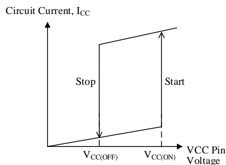
Figure 9-3. Relationship between VCC Pin Voltage and I CC
