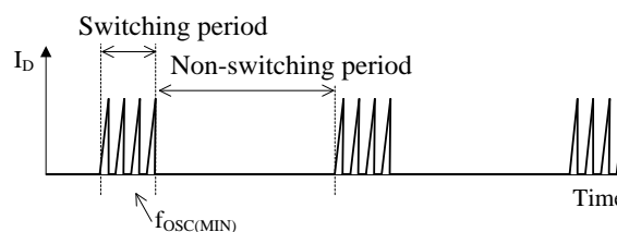
Figure 9-12. Switching Waveform at Burst Oscillation
