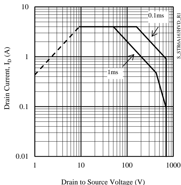
Figure 3-5. STR6A163HVD SOA Curve
