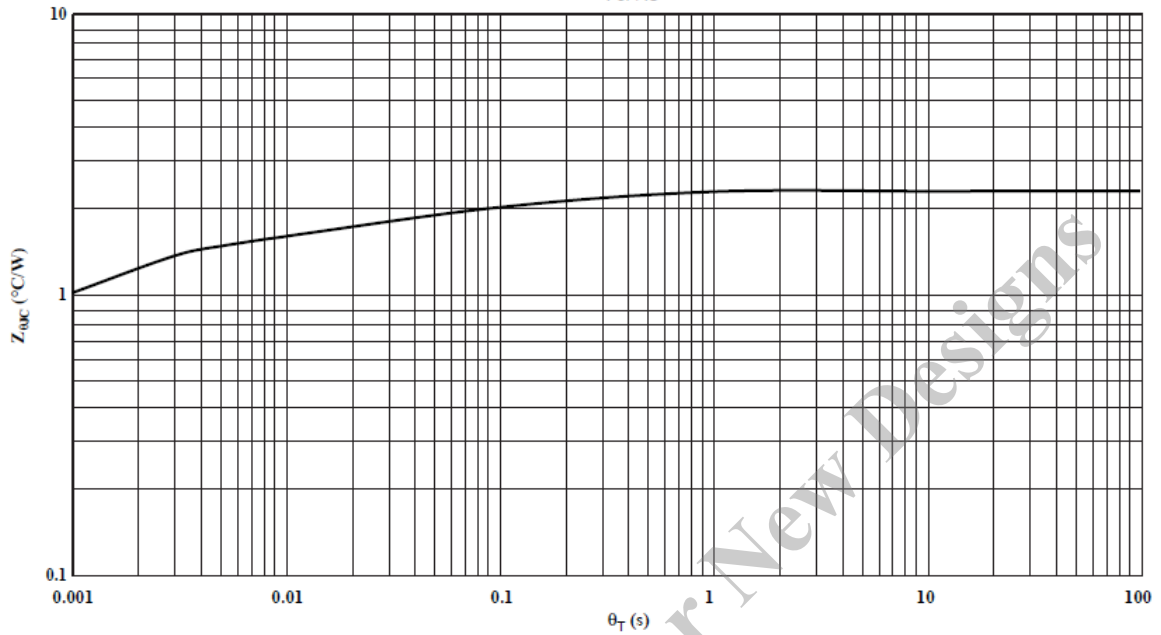
Transient Thermal Impedance versus Triac Voltage Pulse Duration For AC
