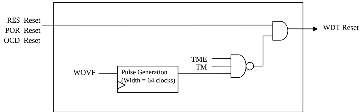
Figure 16-2. Reset Configuration
