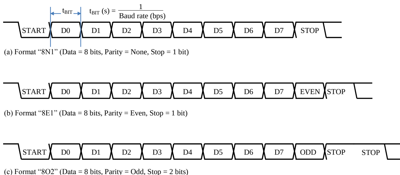
Figure 28-7. UART Character Formats Example
