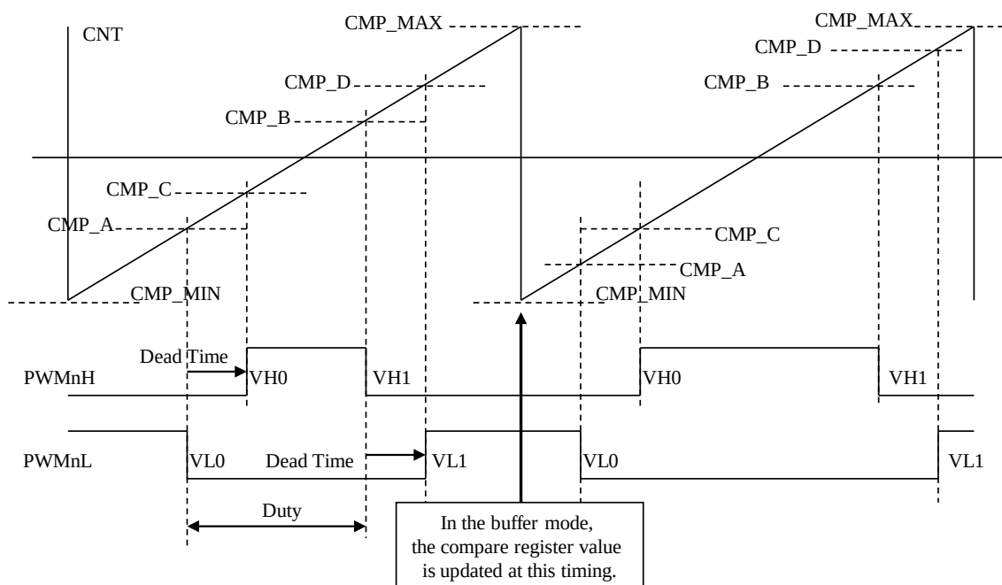
Figure 15-2. PWM Mode 0 (Up Mode)
