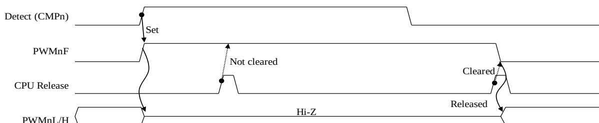
(b) CPU Release (POCCR n .EN = 1)
