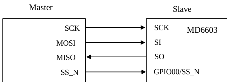
Figure 18-10. Connection in Slave Mode (Slave Device: MD6603)
