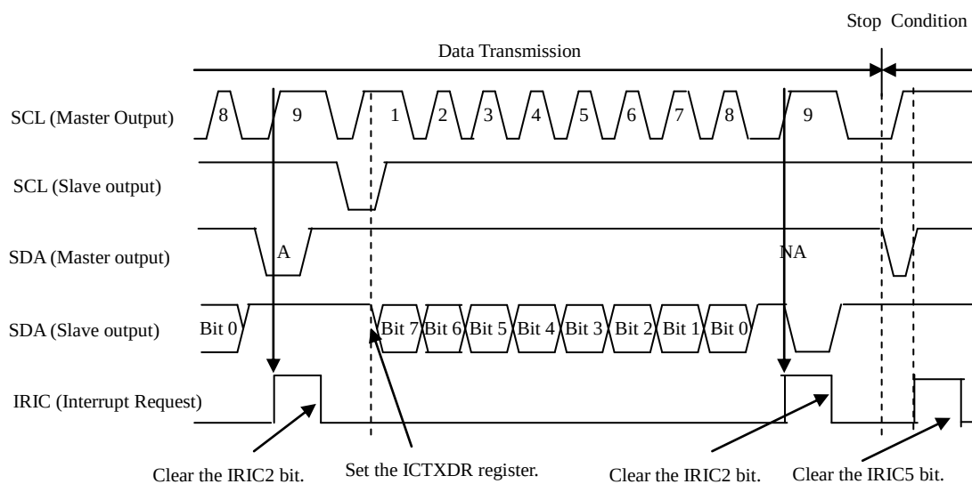
Figure 19-9. Slave Transmission Timing
