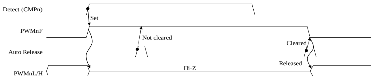
(a) Auto-release (POCCR n .EN = 1, POCCR n .ARELEN = 1)
