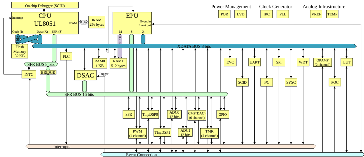
Figure 2-1. Block Diagram
