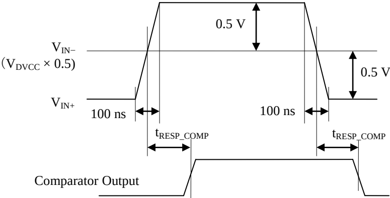
Figure 29-3. Comparator Timing
