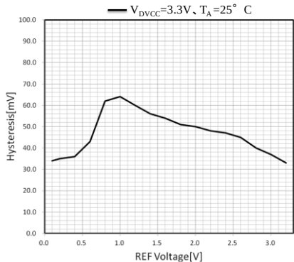
Figure 29-2. Comparator Hysteresis
