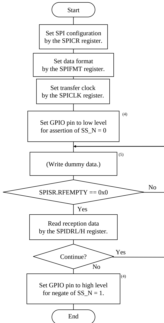
Figure 18-12. Master Mode (Reception)
