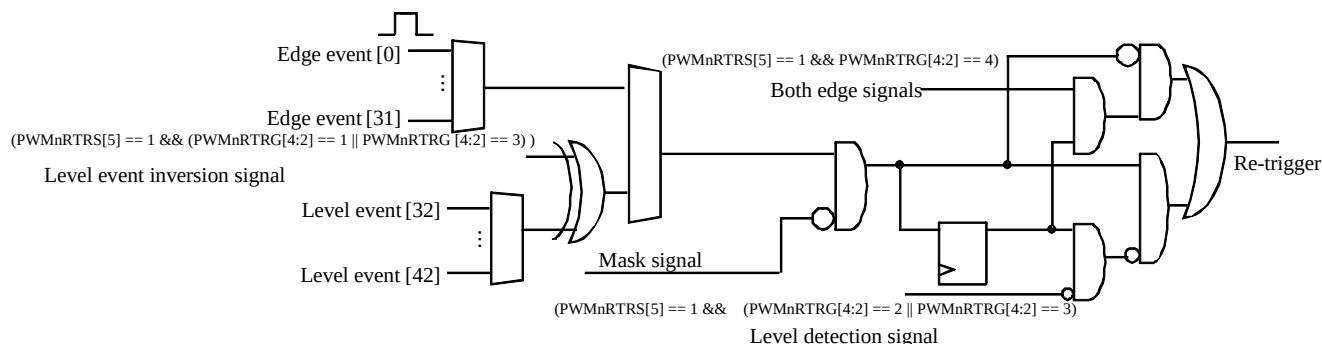
Figure 15-15. Re-trigger Detection Circuit
