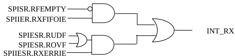
Figure 18-4. INT_RX Generation Logic
