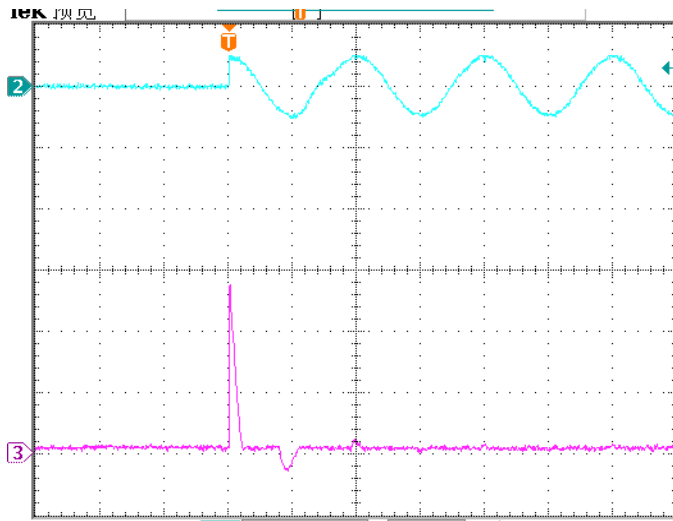
図15 突入電流波形 Fig.15 Inrush Current Waveform
