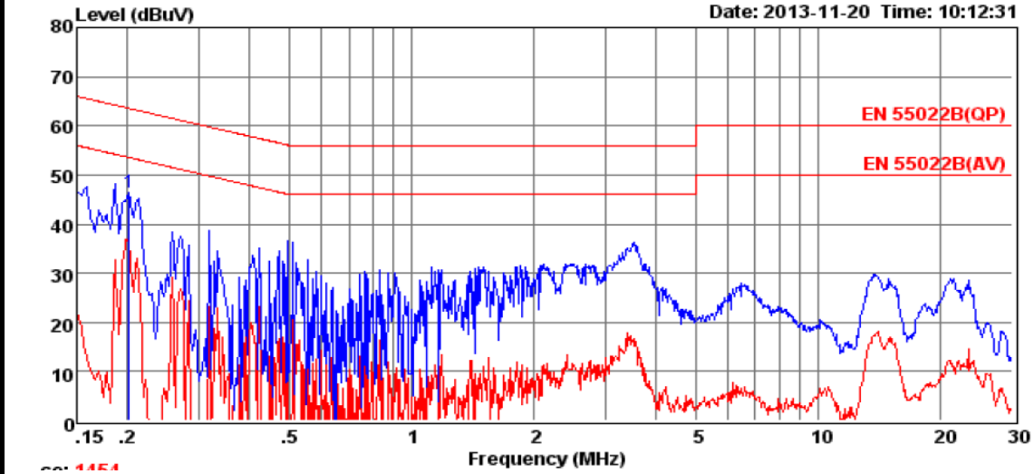
図18 雑音端子電圧 Fig.18 Conduction Noise Waveform
