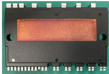
Figure 3. Oxidation 1
