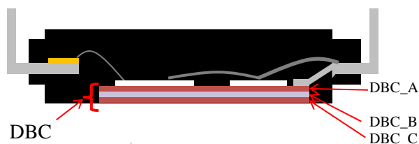
Figure 1. DBC Structure
