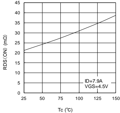
RDS(ON)-Tc characteristics (typical) ID=7.9A, VGS=4.5V
