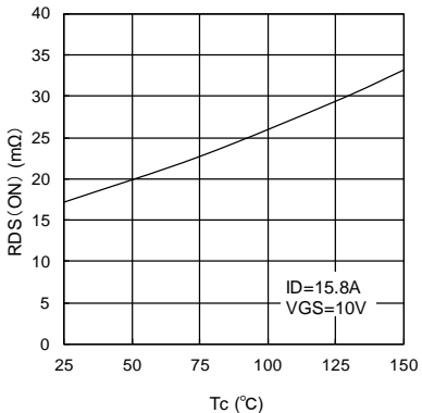
RDS(ON)-Tc characteristics (typical) ID=15.8A, VGS=10V
