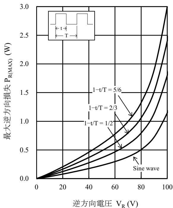
図4 P_{R(MAX)} - V_R 特性 ( T_J = 150\text{ }^{\circ}\text{C} )
