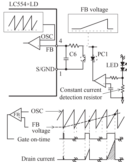
Figure 11. On-time control
