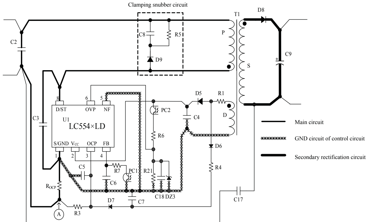
Figure 35. An example schematic of a typical application circuit
