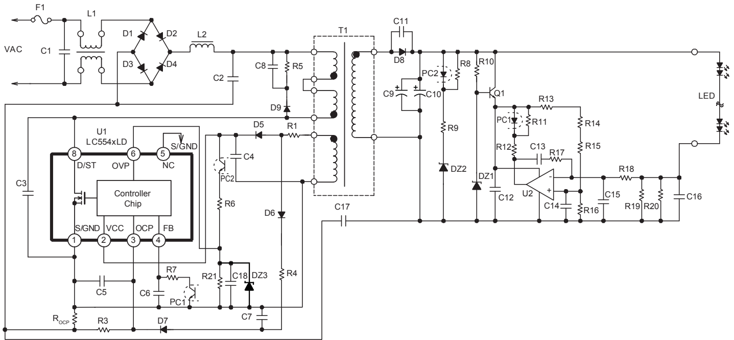
Power supply circuit example for LED lighting
