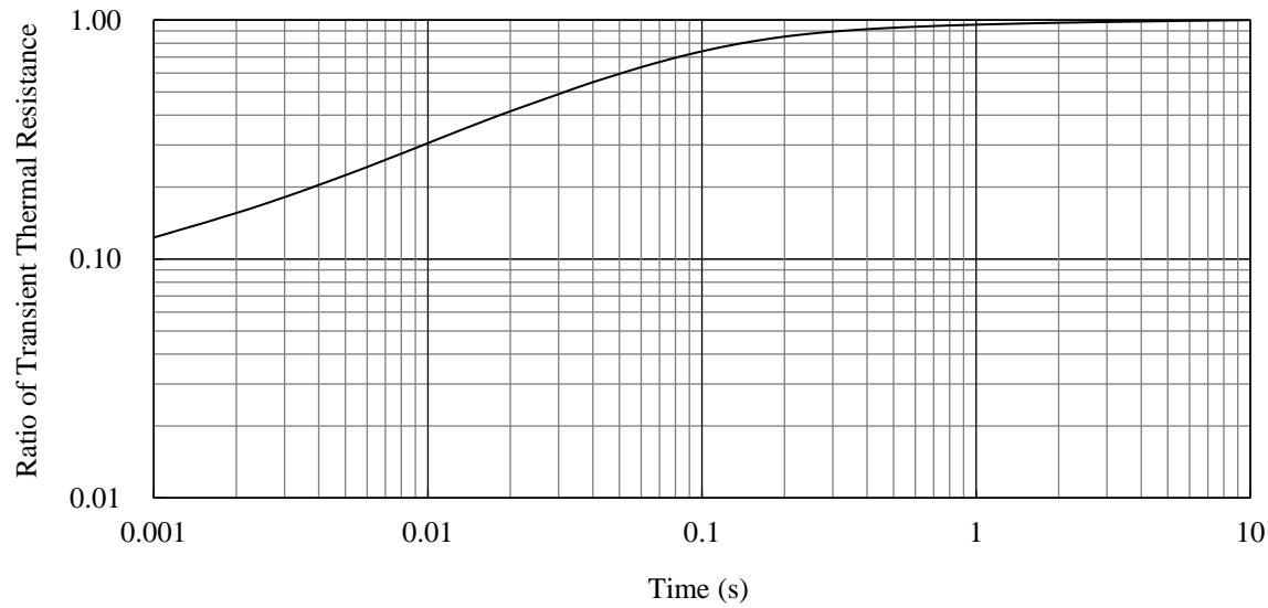
Figure 16-1. Transient Thermal Resistance
