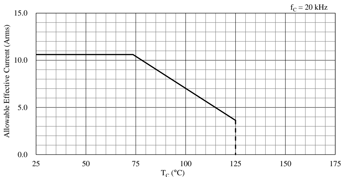
Figure 16-7. Allowable Effective Current ( f_c = 20 kHz)
