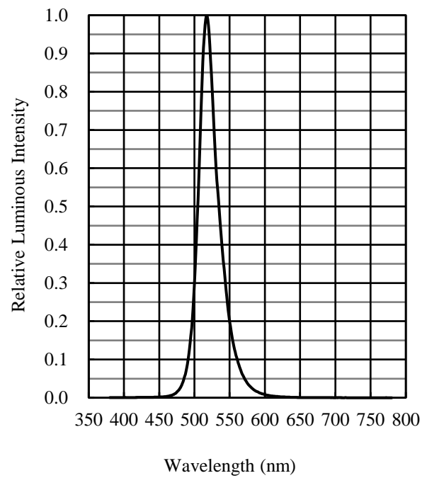
Figure 5. Spectrum
