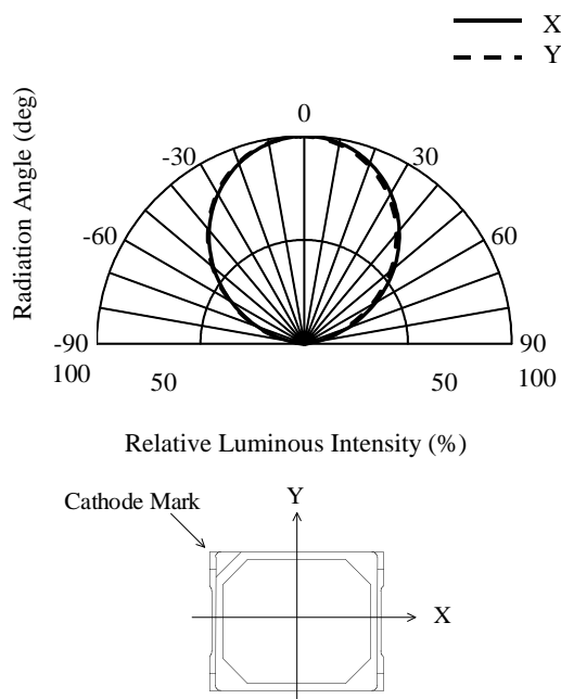
Figure 6. Directivity
