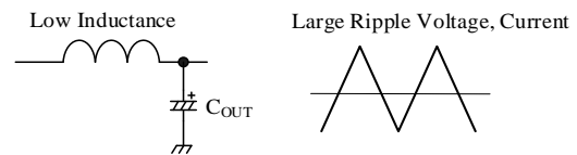
Figure 11-2. Ripple Voltage and Current (Low Inductance)
