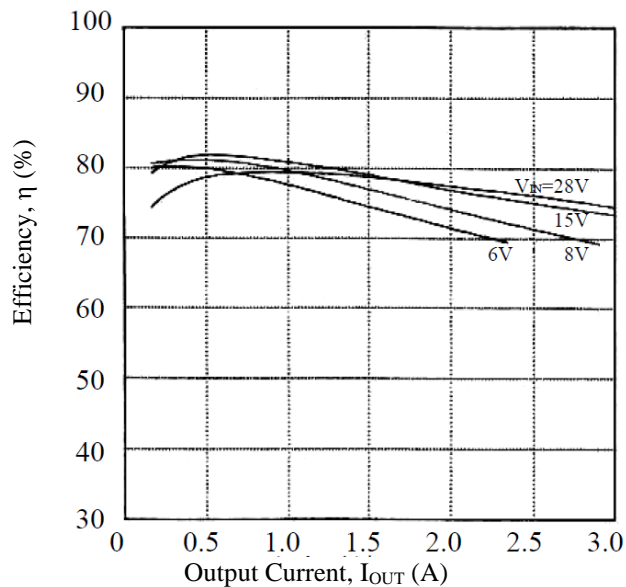
Figure 13-1. Efficiency
