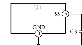
Figure 10-8. Soft Start Function
