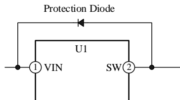
Figure 11-9. Addition of Reverse Bias Protection Diode
