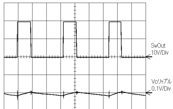
Figure 11-8. With Noise Reduction Circuit
