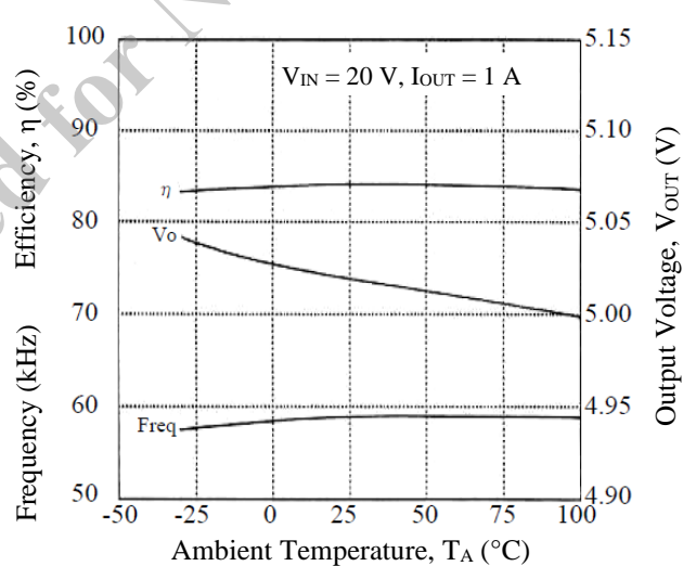
Figure 13-12. Temperature Characteristic
