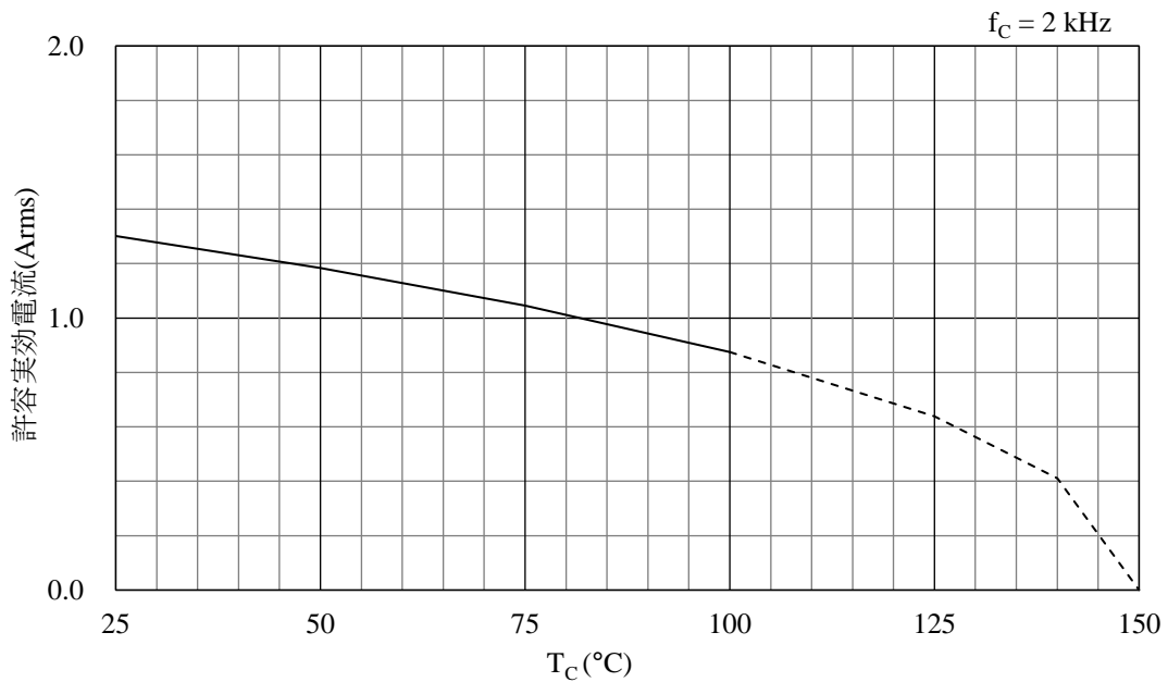
Figure 15-31. Allowable Effective Current ( f_c = 2\text{ kHz} )
