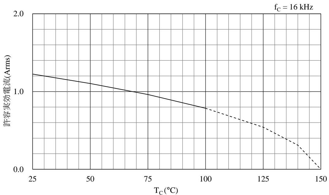
Figure 15-32. Allowable Effective Current ( f_c = 16\text{ kHz} )
