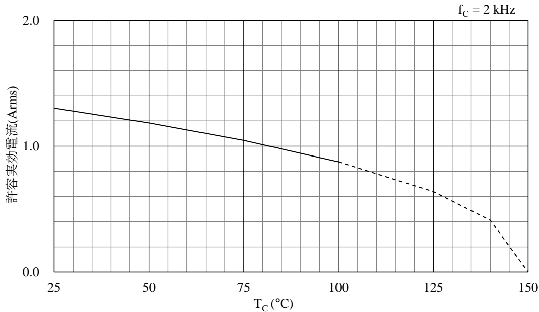
Figure 15-31. Allowable Effective Current ( f_C = 2\text{ kHz} )
