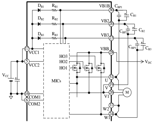
Figure 12-1. Bootstrap Circuit
