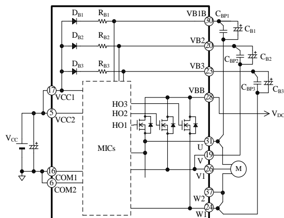
Figure 12-1. Bootstrap Circuit
