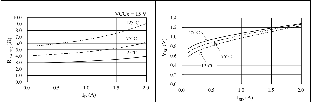
Figure 15-27. Power MOSFET R_{DS(ON)} vs. I_D
