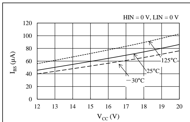
Figure 15-5. Logic Supply Current in 1-phase Operation ( H_{INx} = 0 V), I_{BS} vs. V<sub>B</sub> Pin Voltage, V_B
