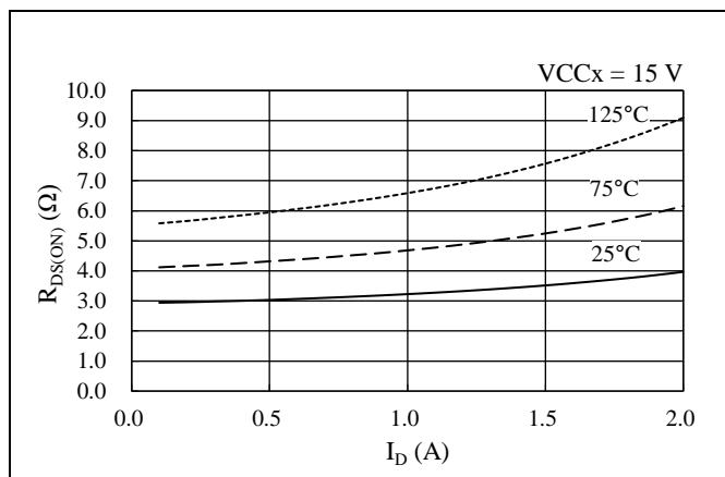
Figure 15-27. Power MOSFET R_{DS(ON)} vs. I_D
