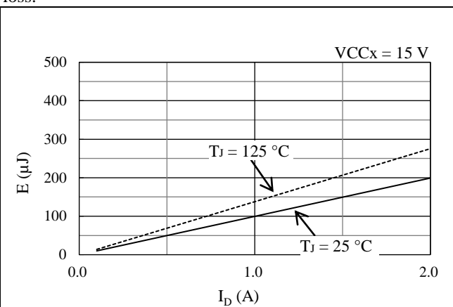
Figure 15-30. Low-side Switching Loss
