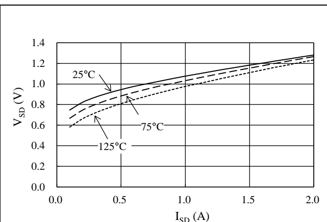
Figure 15-28. Power MOSFET V_{SD} vs. I_{SD}
