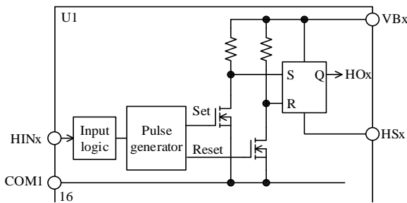
Figure 12-2. Internal Level-shifting Circuit
