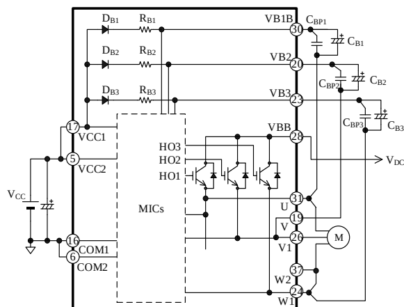
Figure 12-1. Bootstrap Circuit
