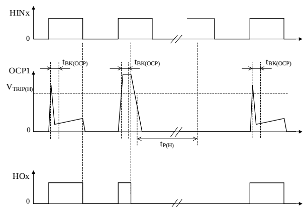
Figure 12-15. OCP1 Operational Waveforms
