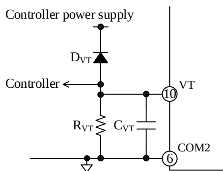
Figure 12-10. VT Pin Peripheral Circuit
