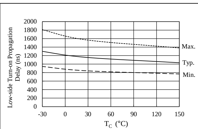
Figure 15-16. Low-side Turn-on Propagation Delay vs. T_C (from LINx to LOx)
