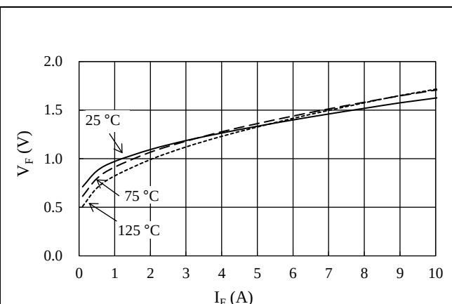
Figure 15-27. FRD V_F vs. I_F
