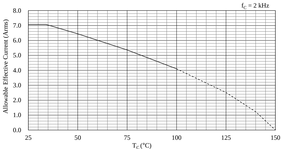
Figure 15-30. Allowable Effective Current ( f_C = 2 kHz)
