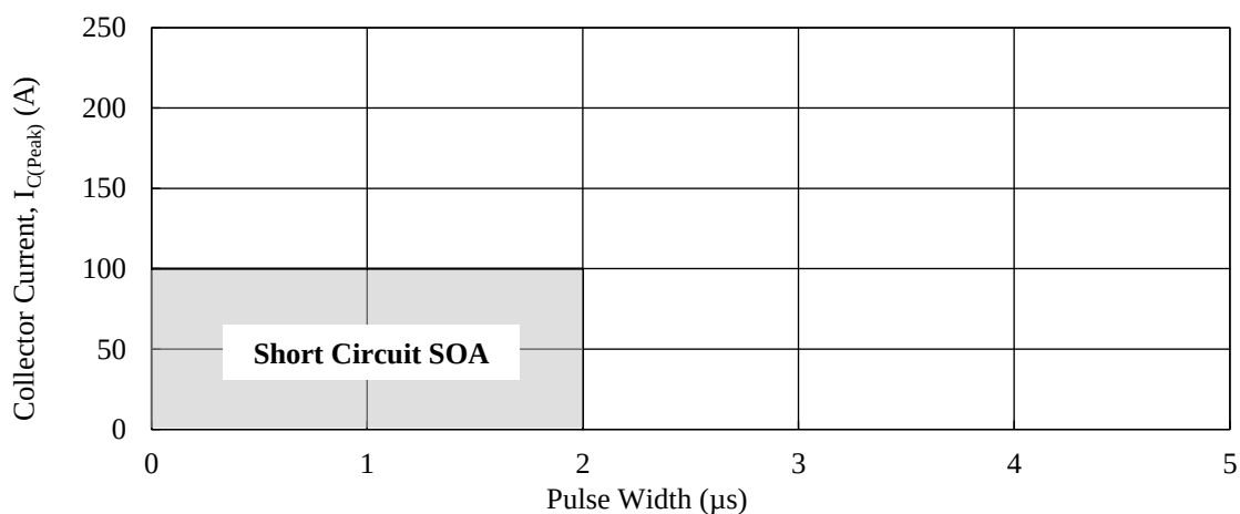
Figure 15-33. Short Circuit SOA
