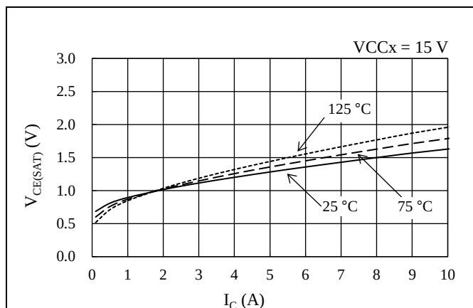
Figure 15-26. IGBT V_{CE(SAT)} vs. I_C
