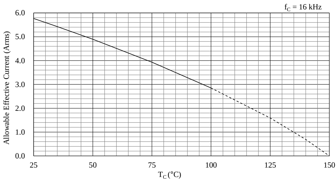
Figure 15-31. Allowable Effective Current ( f_C = 16 kHz)
