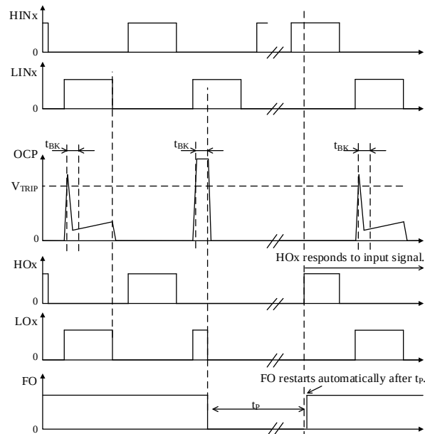
Figure 12-17. OCP2 Operational Waveforms
