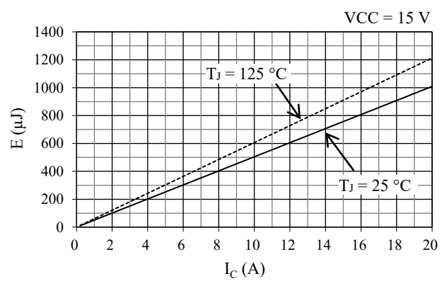
Figure 15-4. Low-side Switching Loss
