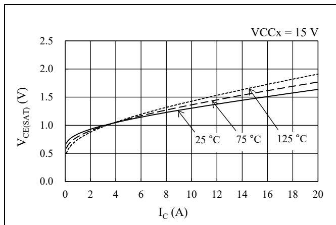
Figure 15-1. IGBT V_{CE(SAT)} vs. I_C
