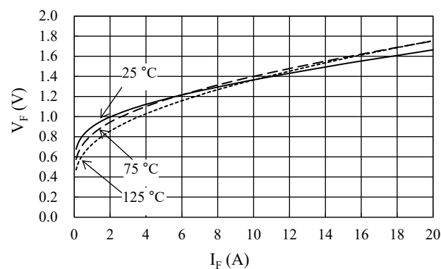
Figure 15-2. Freewheeling Diode V_F vs. I_F
