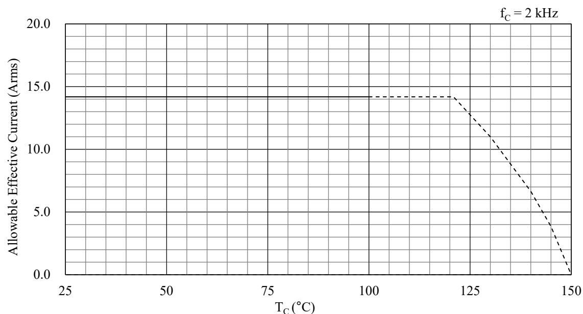
Figure 15-5. Allowable Effective Current ( f_C = 2 kHz)
