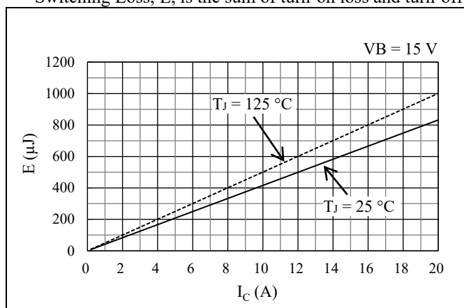
Figure 15-3. High-side Switching Loss
