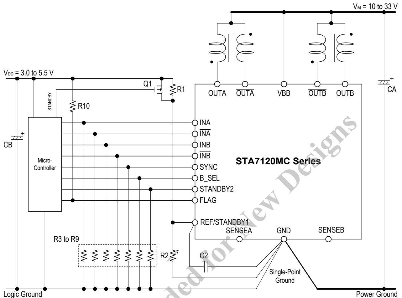
Figure 8-1. Application Example
