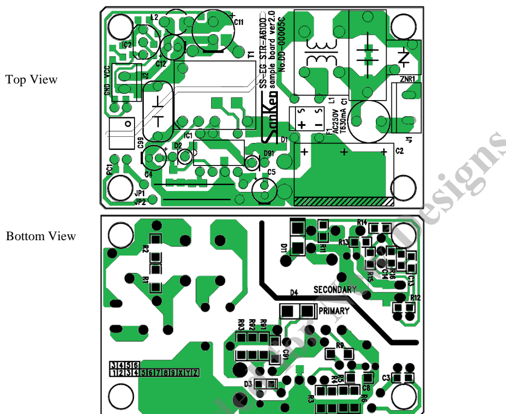
Figure 11-1. PCB Layout Example
