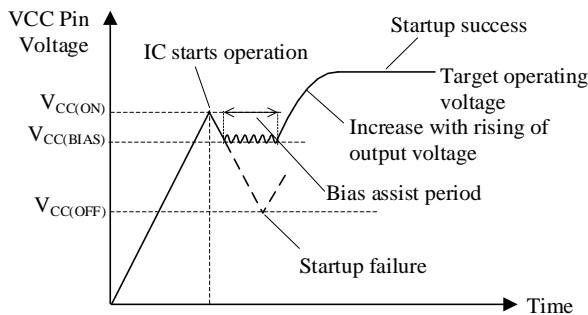
Figure 10-3. VCC Pin Voltage during Startup Period
