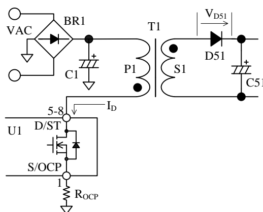
Figure 10-10. Flyback Control Circuit
