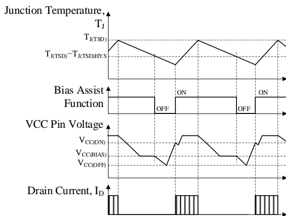
Figure 10-18. TSD Operational Waveforms
