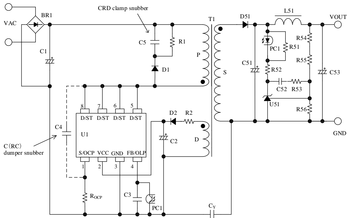
Figure 7-1. Typical Application
