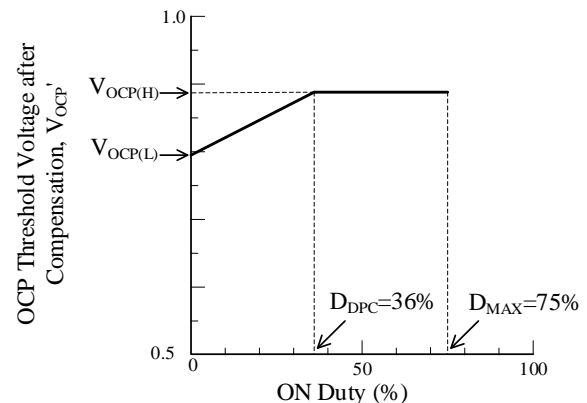
Figure 10-14. Relationship between Duty Cycle and Drain Current Limit after Compensation
