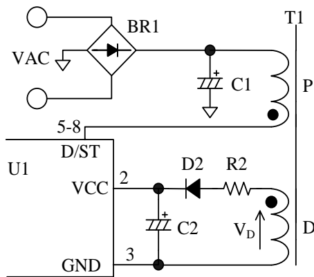
Figure 10-1. VCC Pin Peripheral Circuit
