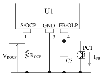
Figure 10-5. FB/OLP Pin Peripheral Circuit
