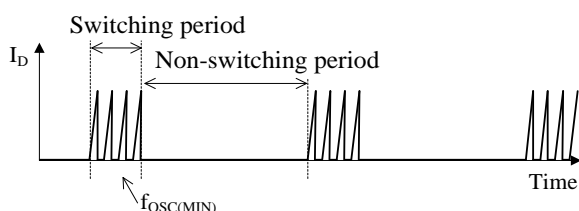
Figure 10-9. Switching Waveform at Burst Oscillation
