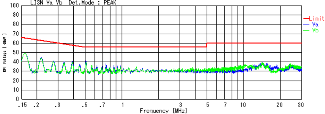
図20 雑音端子電圧 Fig.20 Conduction Noise Waveform
