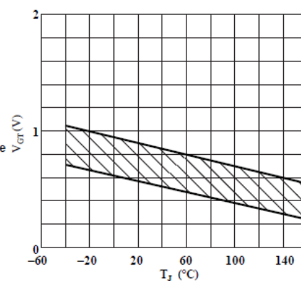
Typical Gate Trigger Voltage versus Junction Temperature at V_D = 6 V and R_L = 10\ \Omega
