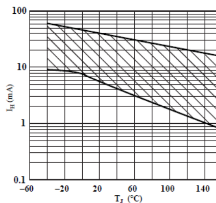
Typical Holding Current versus Junction Temperature at R_{GREF} = 10\ \text{k}\Omega
